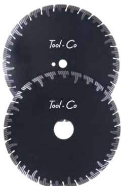
TURBO SEGMENTED WET CUTTING Our BBR350 diamond blades are designed to cut Natural Stone and Quartz on lower power machines rated around 2200W
